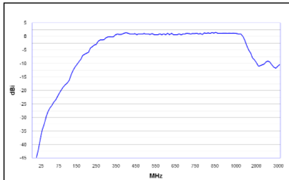
Gain Diagram BicoLOG 20300
